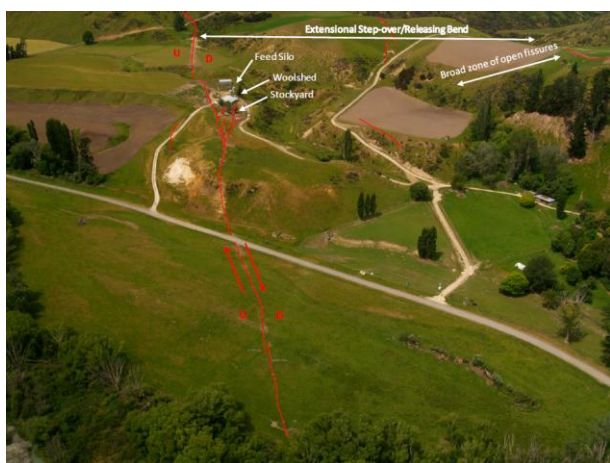
Figure 4: Aerial view of The Humps Fault surface rupture (red lines) at Glenbourne Farm, showing the sense of movement (red arrows) and highlighting farm infrastructure damaged by the earthquake (Lat 42.615°S, Lon 173.105°E; view northeast; photo and annotation by Clark Fenton).
