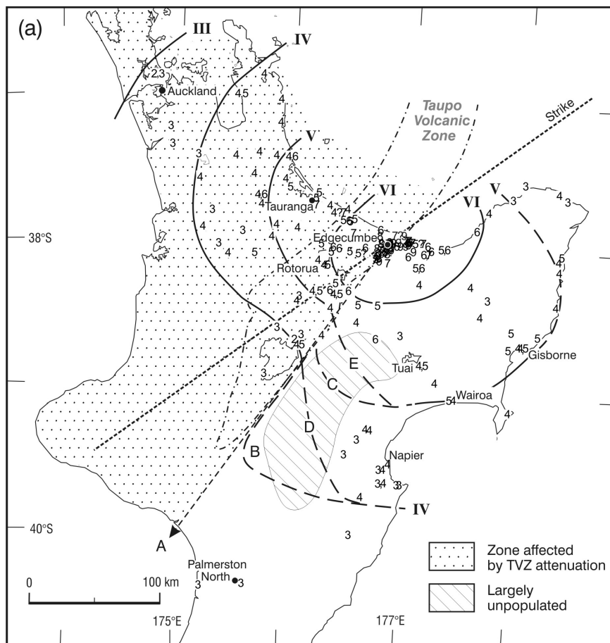
Figure 7a. Revised isoseismal map of the 1987 Edgecumbe earthquake, (a) overall map.
