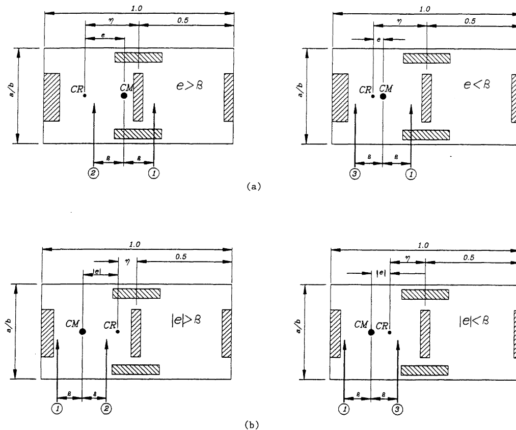
Figure 12 Loading cases to evaluate the edge displacement criterion
