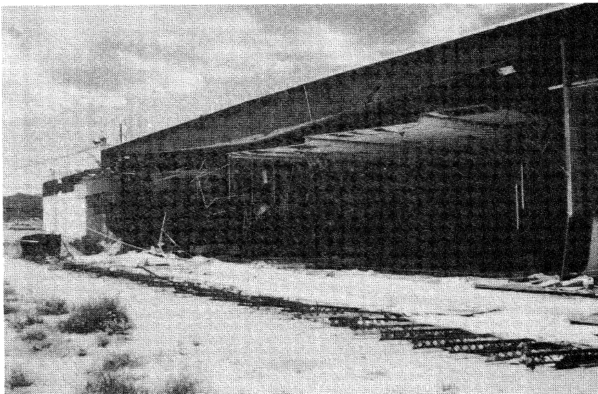
Figure 10. Collapsed east wall of the bowling alley in the eastern part of the town of Yucca Valley. Steel roof beams were not significantly damaged, but many false ceiling panels have fallen. The west wall of the building was constructed of concrete blocks that suffered only minor cracking. Location shown on Fig 5.
