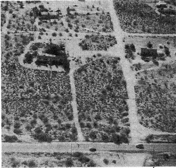
Figure 7. Aerial view of the Johnson Valley fault (7A), parallel and about 50 m east of California Highway 247 (foreground). Note the complex nature of surface faulting, and occurrence of cracks running at a high angle to the fault. Fig 7B shows a fence displaced 2.7 m right-lateral on the Johnson Valley fault in the same vicinity. At this site displacement occurred on two principal fractures in a deformation zone about 5 m wide. Location shown on Fig. 5.
