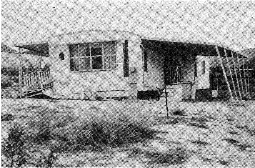
Figure 11. Damaged trailer house about 100 m west of the Johnson Valley fault. The trailer was apparently poorly tied to its wooden pile foundation. Location shown in Fig 5.
