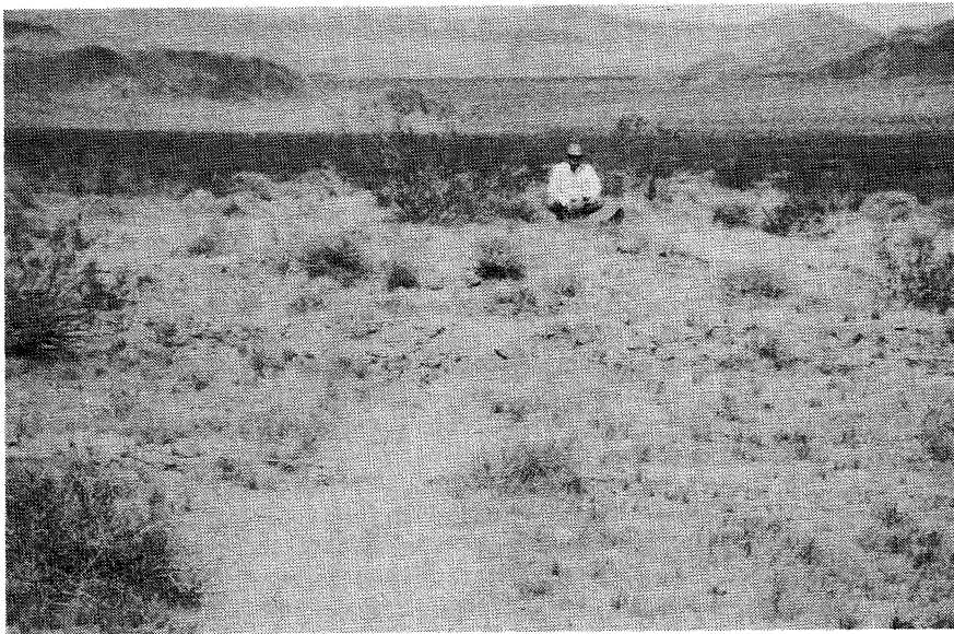
Figure 8. Off-road motorcycle track displaced by 4.5 m right-lateral on the Emerson fault. Displacement occurs across four principal fractures, most of which also have minor upthrow to the east. Photograph taken looking east; location is shown on Fig 5.
