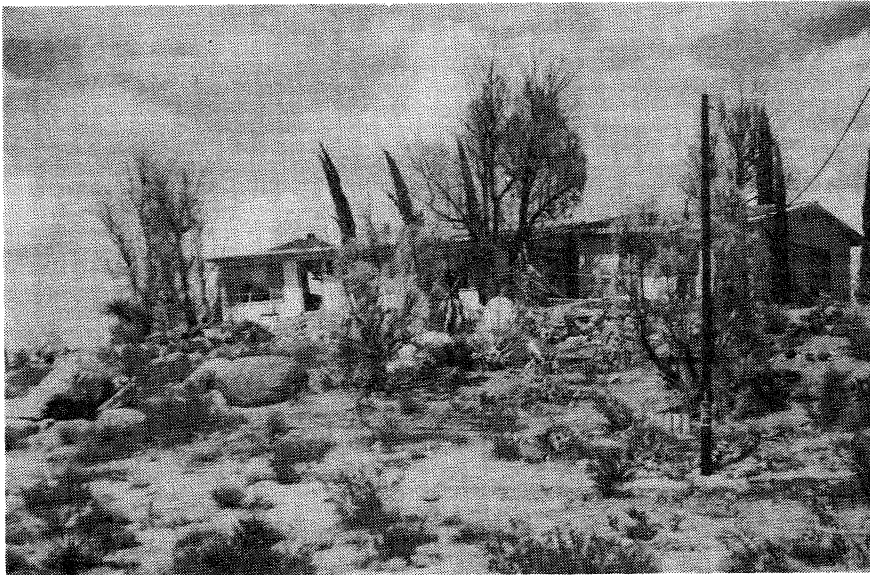
Figure 12. Exterior view of severely damaged "hilltop" house located about 60 m east of the Johnson Valley fault. Note that several trees have died (photo taken about two weeks following the earthquake) because of root damage. Location shown on Fig 5.
