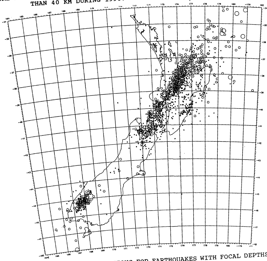
URE 2. PRELIMINARY LOCATIONS FOR EARTHQUAKES WITH FOCAL DEPTHS LESS THAN 40 KM DURING 1990.
