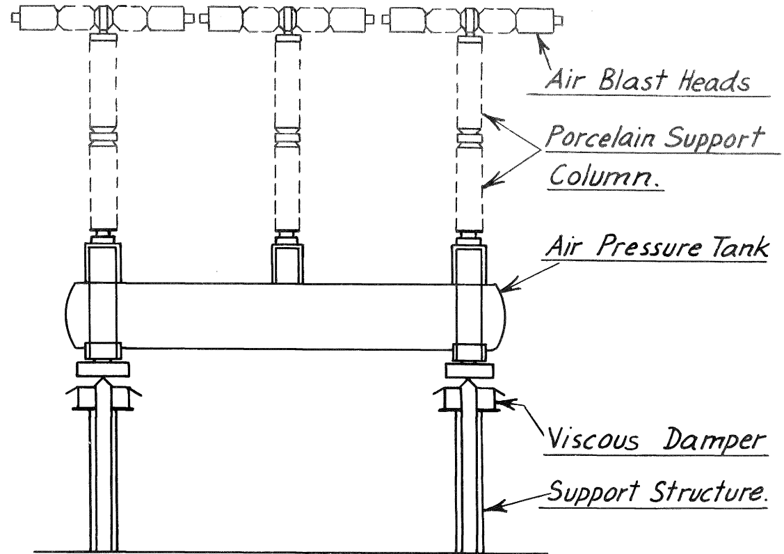
Single Pole of Circuit Breaker
