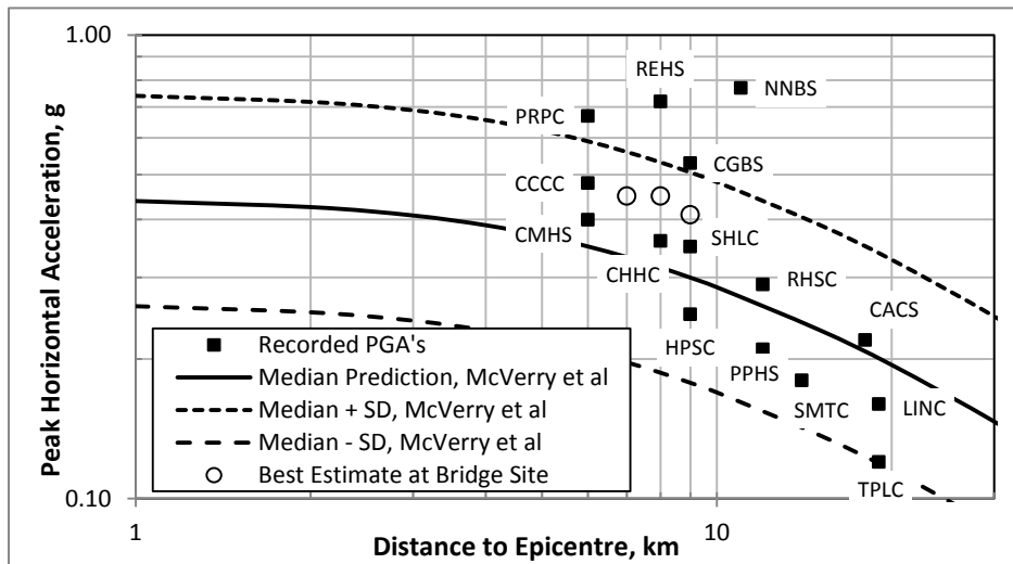
Figure 5: Recorded PGA's in Christchurch earthquake, best estimates for bridge sites and PGA predictions. (McVerry et al, 2006).
