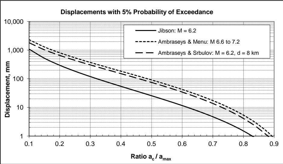
Figure 14: Outward displacements in Christchurch earthquake for 5% probability of exceedance.
