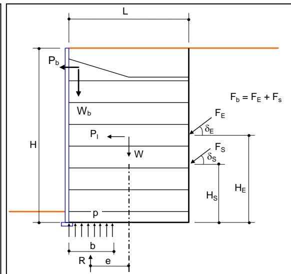
Figure 7: Reinforced Earth block external stability.
