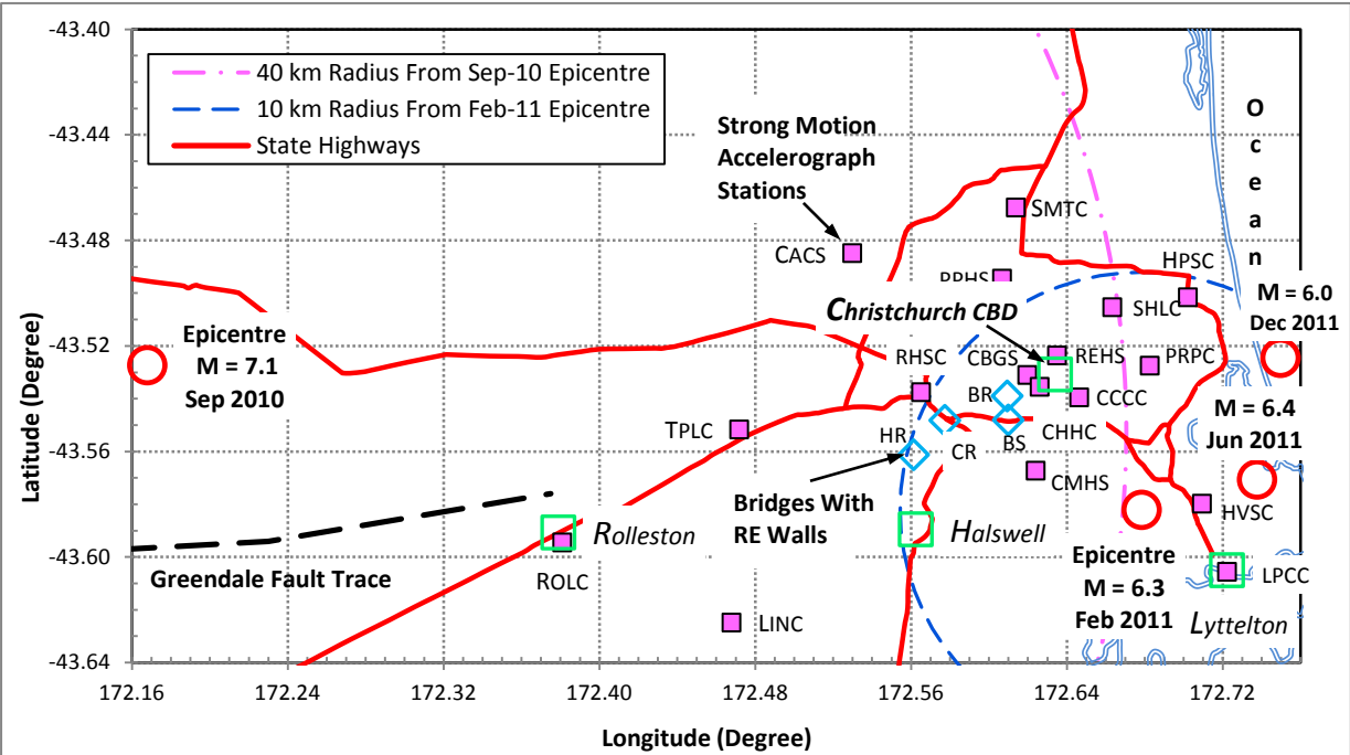
Figure 4: Location of bridges with Reinforced Earth abutments in relation to earthquake epicentres. See Table 5 for bridge name abbreviations.
