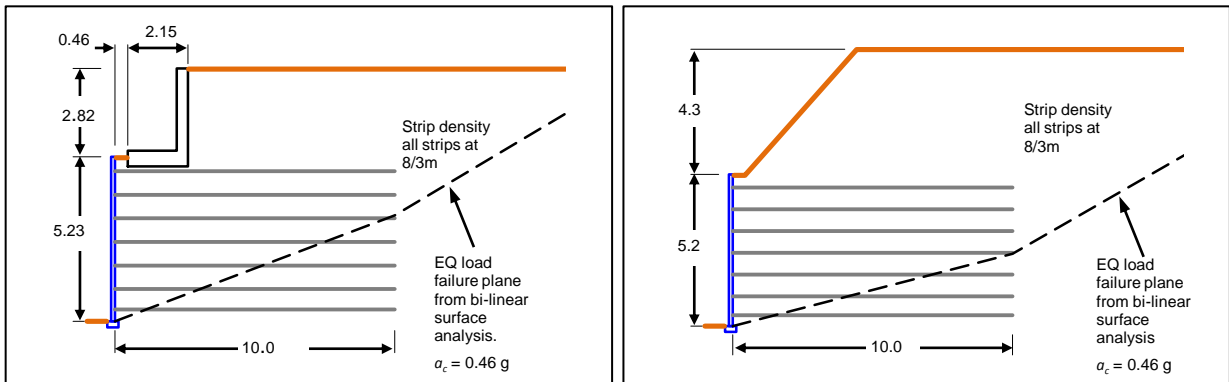
Figure 9: Barrington Street failure planes Section A. Design (left) and Surcharge (right).
