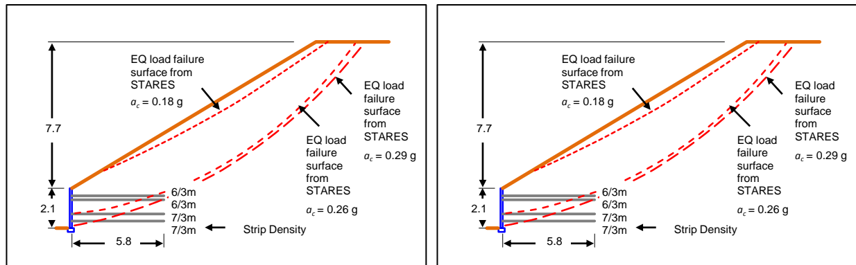
Figure 13: Curletts Road failure planes Section C. Design (left) and Surcharge (right).
