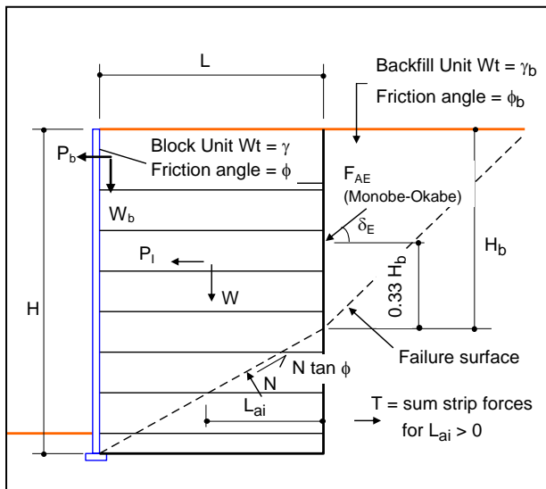
Figure 6: Reinforced Earth block LE analysis.
