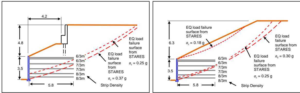
Figure 12: Curletts Road failure planes Section B. Design (left) and Surcharge (right).
