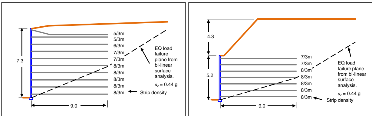
Figure 10: Barrington Street failure planes Section B. Design (left) and Surcharge (right).
