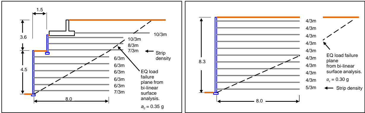
Figure 8: Blenheim Road. Design configuration. Failure planes Section A (left) and B (right)
