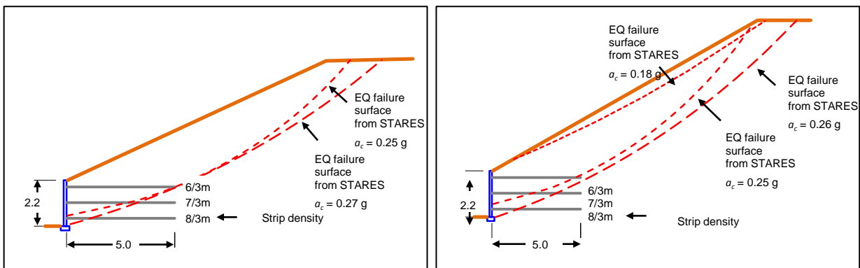
Figure 11: Curletts Road failure planes Section A. Design (left) and Surcharge (right).
