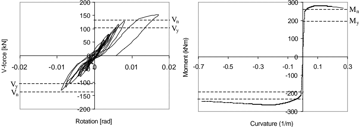
Figure 13 V-force-displacement histories for double-tee beams joint
