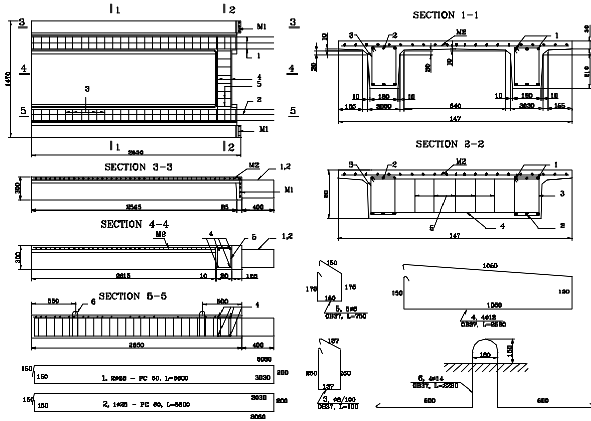
Figure 5 Longitudinal double-tee beam construction details
