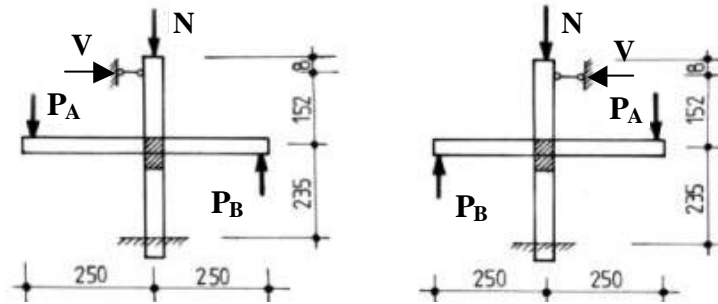
Figure 7 Adopted cyclic loading scheme for test
